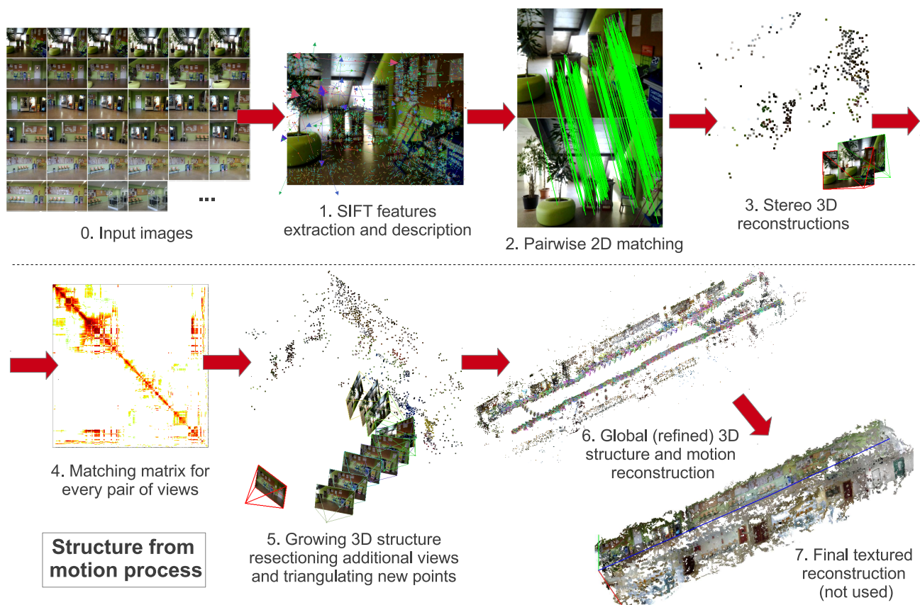
Fig. 2. Illustration of the SfM 3D reconstruction technique. All figures obtained using Wu's VisualSfM software on our test environment (see also sec. VIII).
