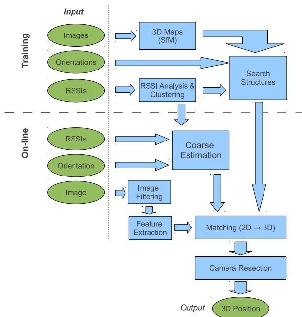
Fig. 1. System overview
