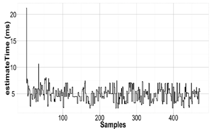
Figure 6. Processing time per test sample (Manhattan distance).
