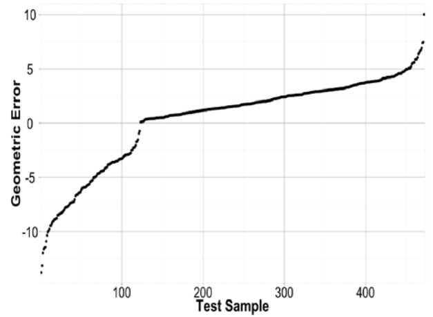
Figure 11. Overall performance of the proposed positioning system ( \alpha = 6 , \beta = 0 , L1 = 100 , N1 = 30 , M1 = 15 , P1 = 7 ).
