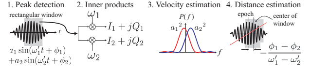
Fig. 3. Overview of the EPAM algorithm
