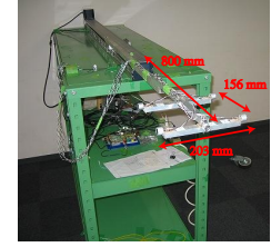
Fig. 8. Five transmitters are moved by the electrical slider
