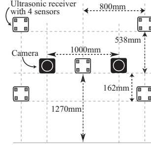
Fig. 11. Arrangement of receiver units and stereo camera
