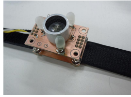
Fig. 6. A marker to be attached to the user (an ultrasonic receiver and three IR-LEDs are mounted)
