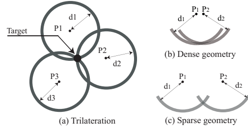
Fig. 1. Trilateration and the effects of the geometric arrangement of measuring nodes
