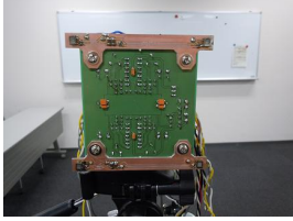
Fig. 5. Ultrasonic receiver unit with four sensors
