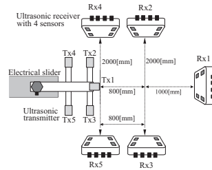
Fig. 7. Experimental setup using an electrical slider
