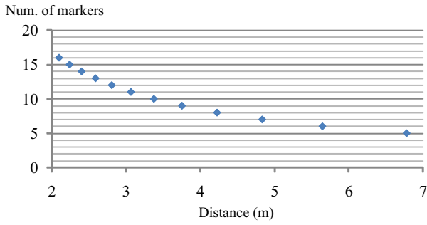
Fig. 4. Maximum numbers of markers by changing distances to receivers
