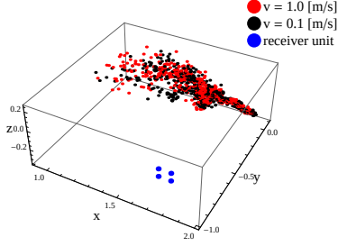
Fig. 9. Tx2's trajectory detected at Rx4
