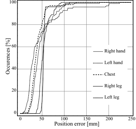
Fig. 12. Error CDF of measured positions of markers
