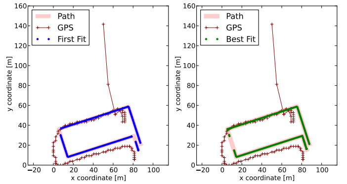
Fig. 7. During the experiment each user walked along a predefined path. In both figures we see the detected steps and their position corresponding to the matching algorithms. GPS was tracked for comparison and is displayed in both figures.
