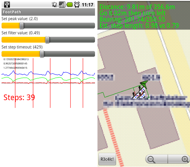
Fig. 5. Screen shots of the calibration screen and during navigation.
